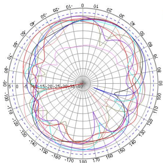
XZ PLANE
