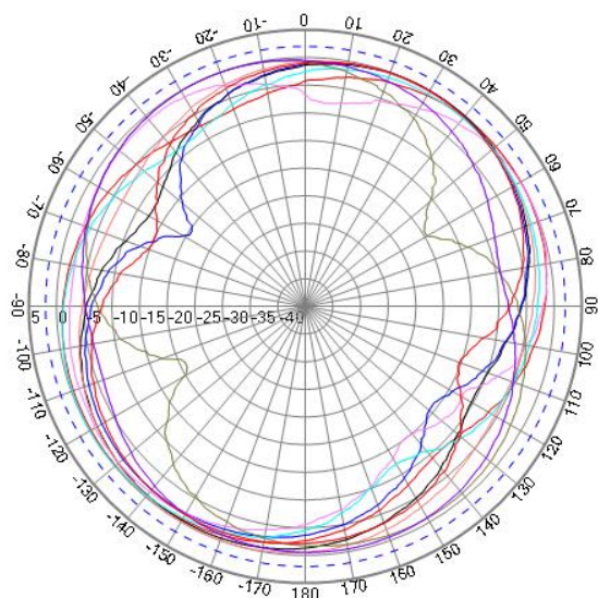
XY PLANE
